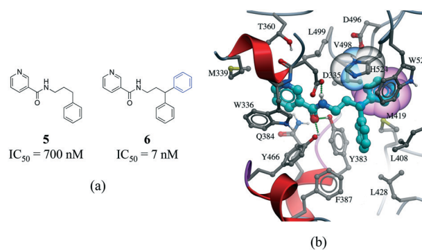
Fig. 7 a) Chemical structure of two inhibitors of human sEH; b) X-ray cocrystal structure of human sEH and 6 (cyan carbons, PDB: 3I1Y). The phenyl ring (transparent CPK magenta) is positioned to allow a \pi -stacking interaction with H524 (shown as transparent CPK). Hydrogen bonds are displayed in dotted green lines.
